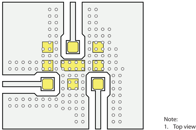
Figure 27. ACMD-7617 Superposed on PCB Layout
