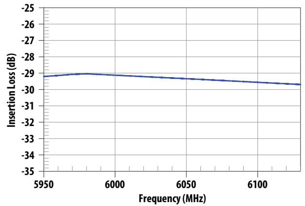
Figure 16. Ant–Rx Rejection, 5950–6130 MHz
