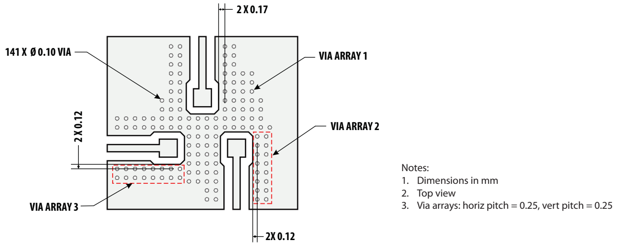
Figure 26. PCB Layout, Via Detail
