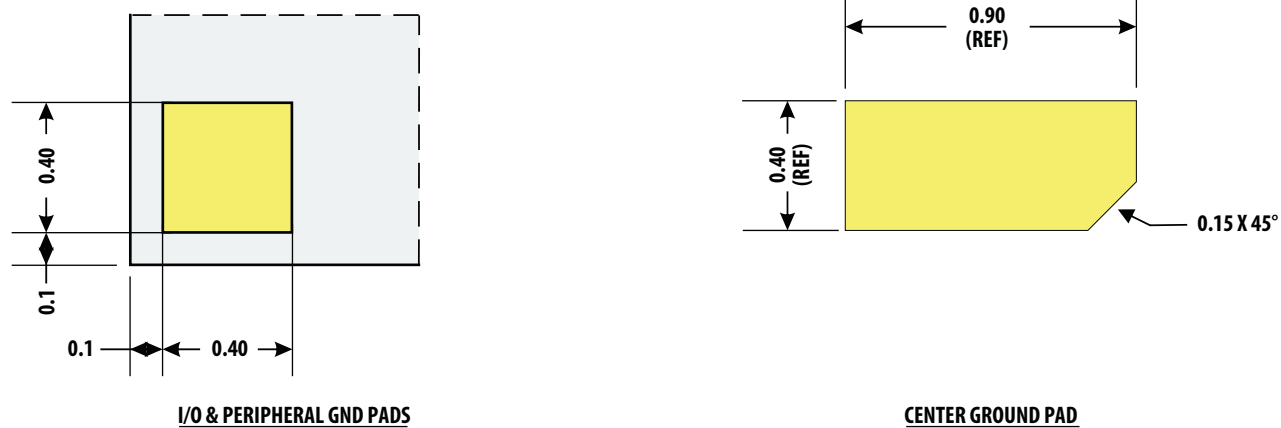
Figure 24. Pad Detail
