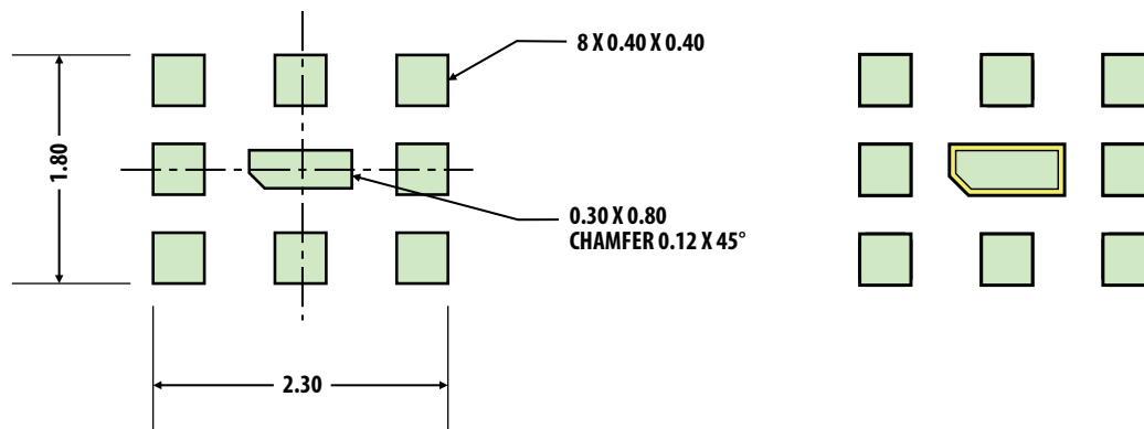
Figure 27. ACMD-7617 Superposed on PCB Layout
