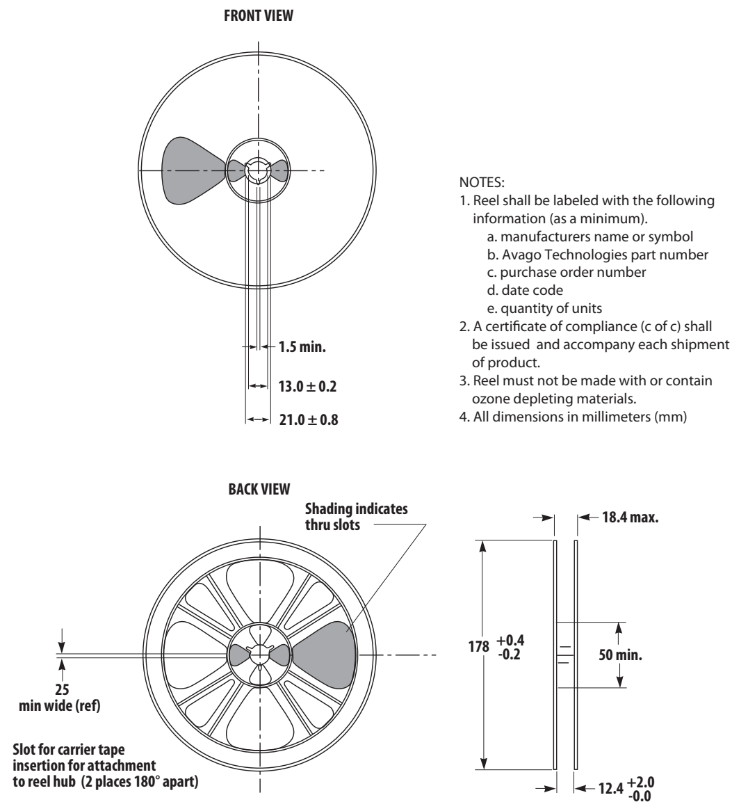
Figure 35. SMT Reel Drawing
